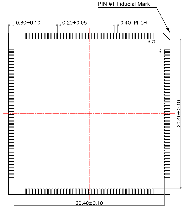
BOTTOM VIEW
